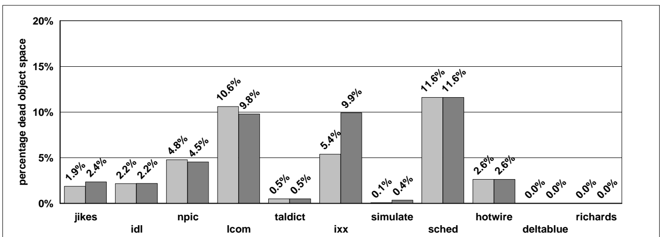
Figure 4: Percentage of object space occupied by dead data members for each of the programs of Table 1. Light grey bars indicate the percentage of space occupied by dead data members throughout program execution. Dark grey bars indicate the reduction of the maximum amount of space (high water mark) required at a single point in time by each program.
