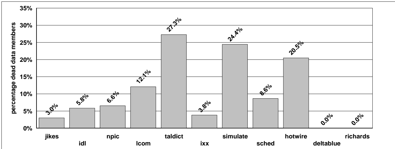
Figure 3: Percentage of dead data members detected in the benchmark programs of Table 1.
